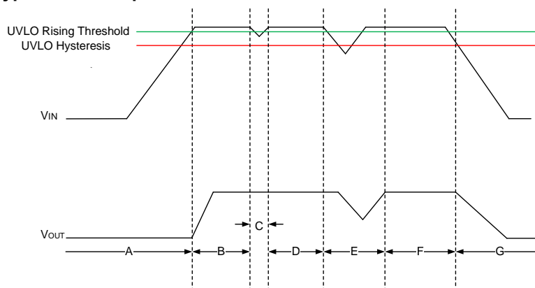
Figure 5-1 Typical UVLO Operation
